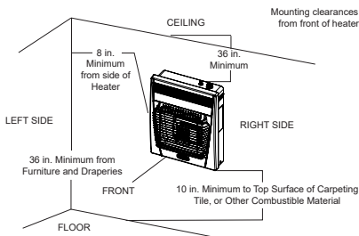
Fig. 9 - Minimum Clearance to Combustible Material Infrared model
